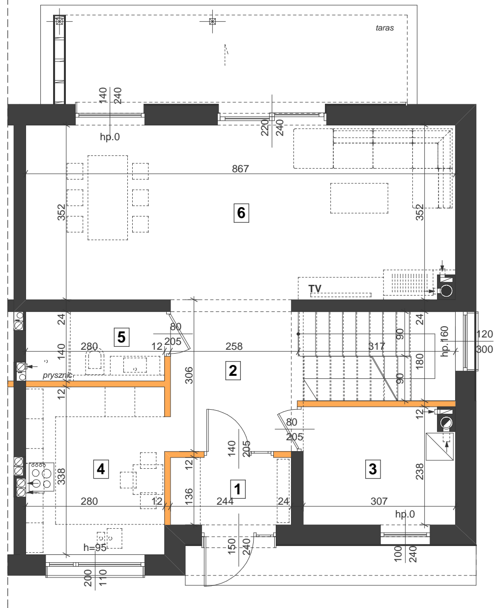
plan parteru
