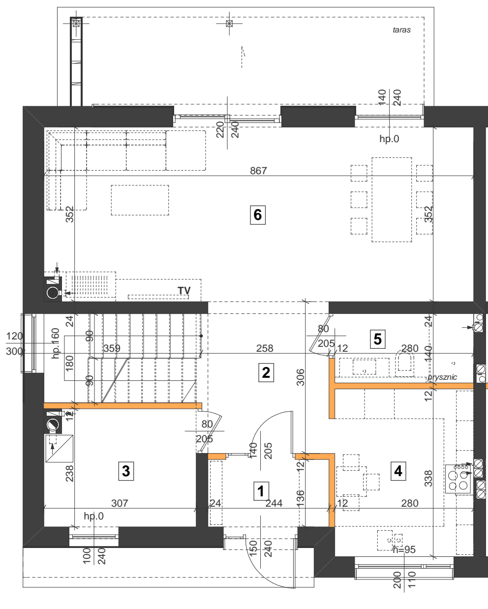
plan parteru
