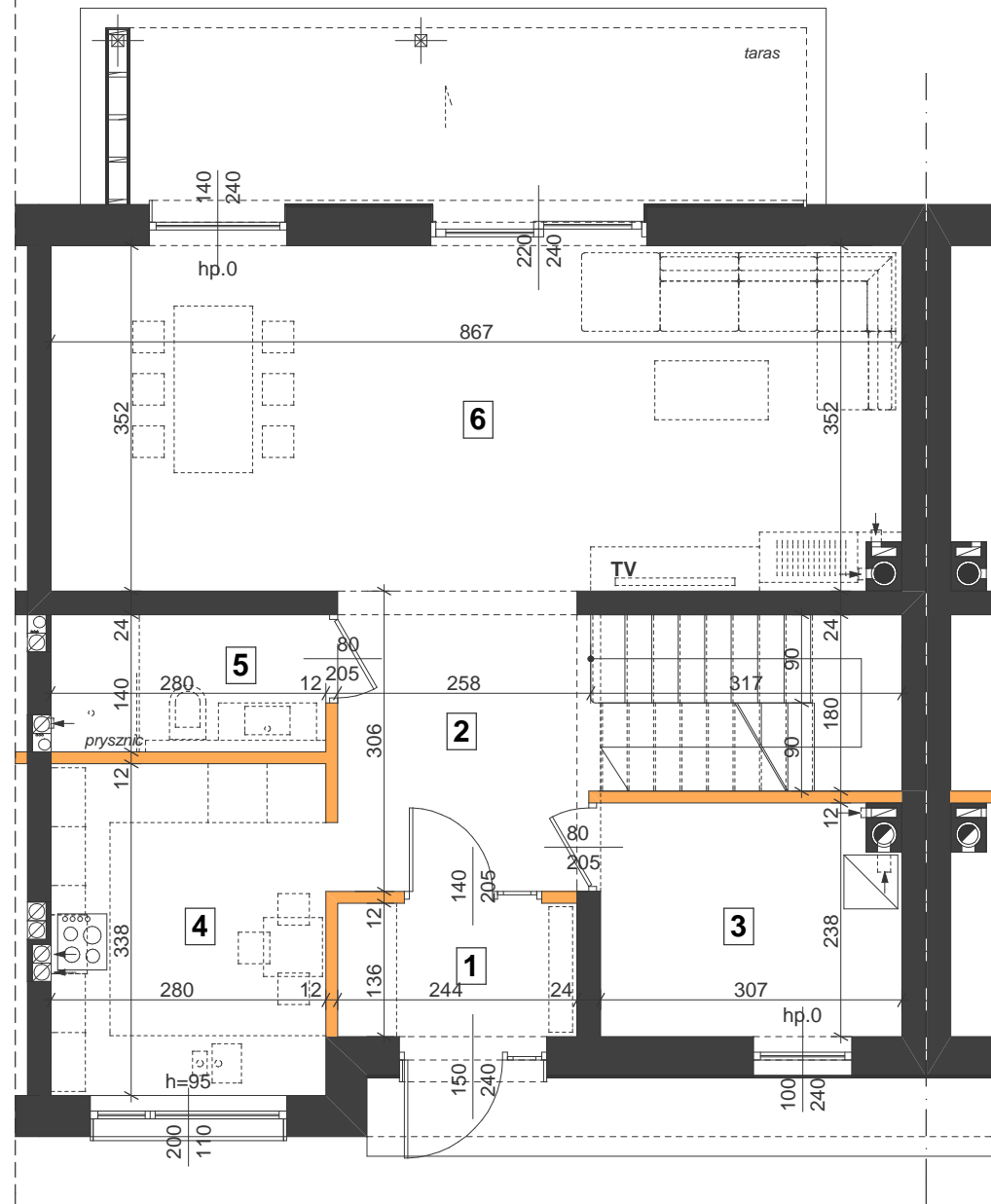
plan parteru
